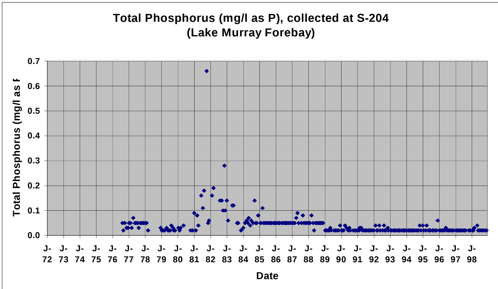
Figure 2-3: Total Phosphorous Concentrations at the Dam Forebay of Lake Murray – 1972 To 1998
